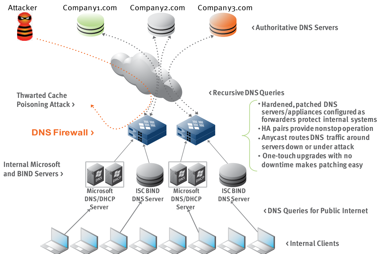
Figure 2: Next Generation Infoblox QuickSecure Design A secure grid of Infoblox appliances configured as forwarders can be added to any existing infrastructure to provide a secure “DNS Firewall” that can be updated quickly, with zero downtime.
